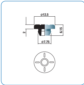
C5422 - Blow back Rough surface
