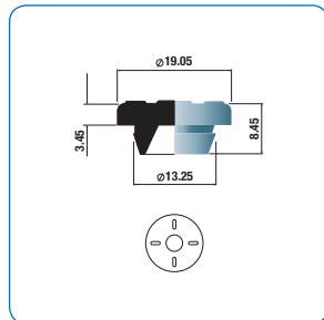
C5474 - Blow back Rough surface
