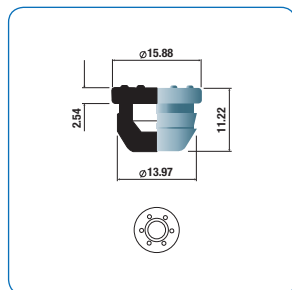
C1584 - Add-vantage stopper
