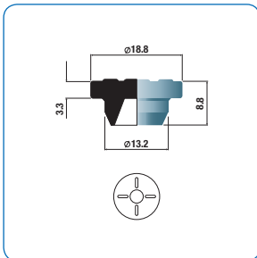
C5394 - ISO 8362 - Non blow back Rough surface
