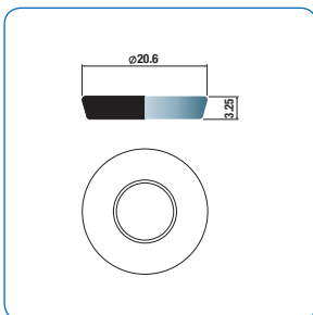
C5510 - Disc Rough surface
